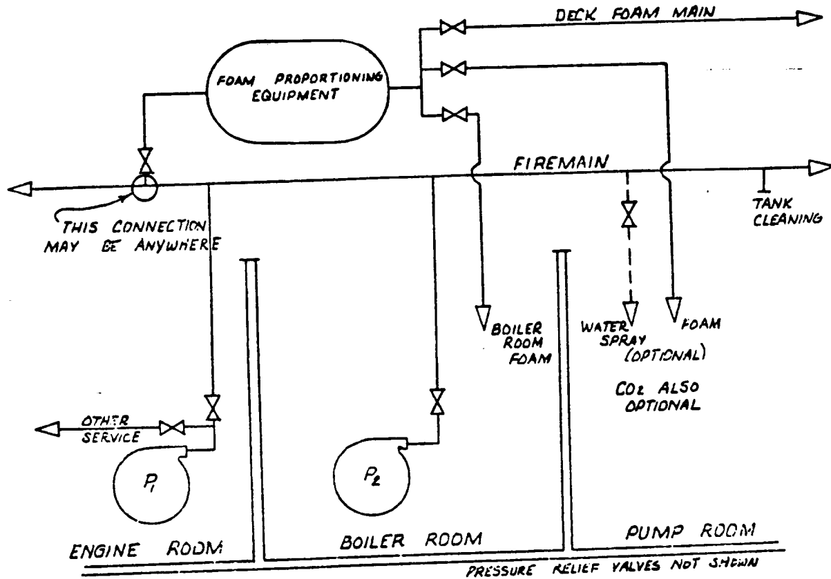
TYPICAL FIREMAIN SYSTEM AS INSTALLED ABOARD TANK VESSEL ALL VALVES NEAR EQUIPMENT
